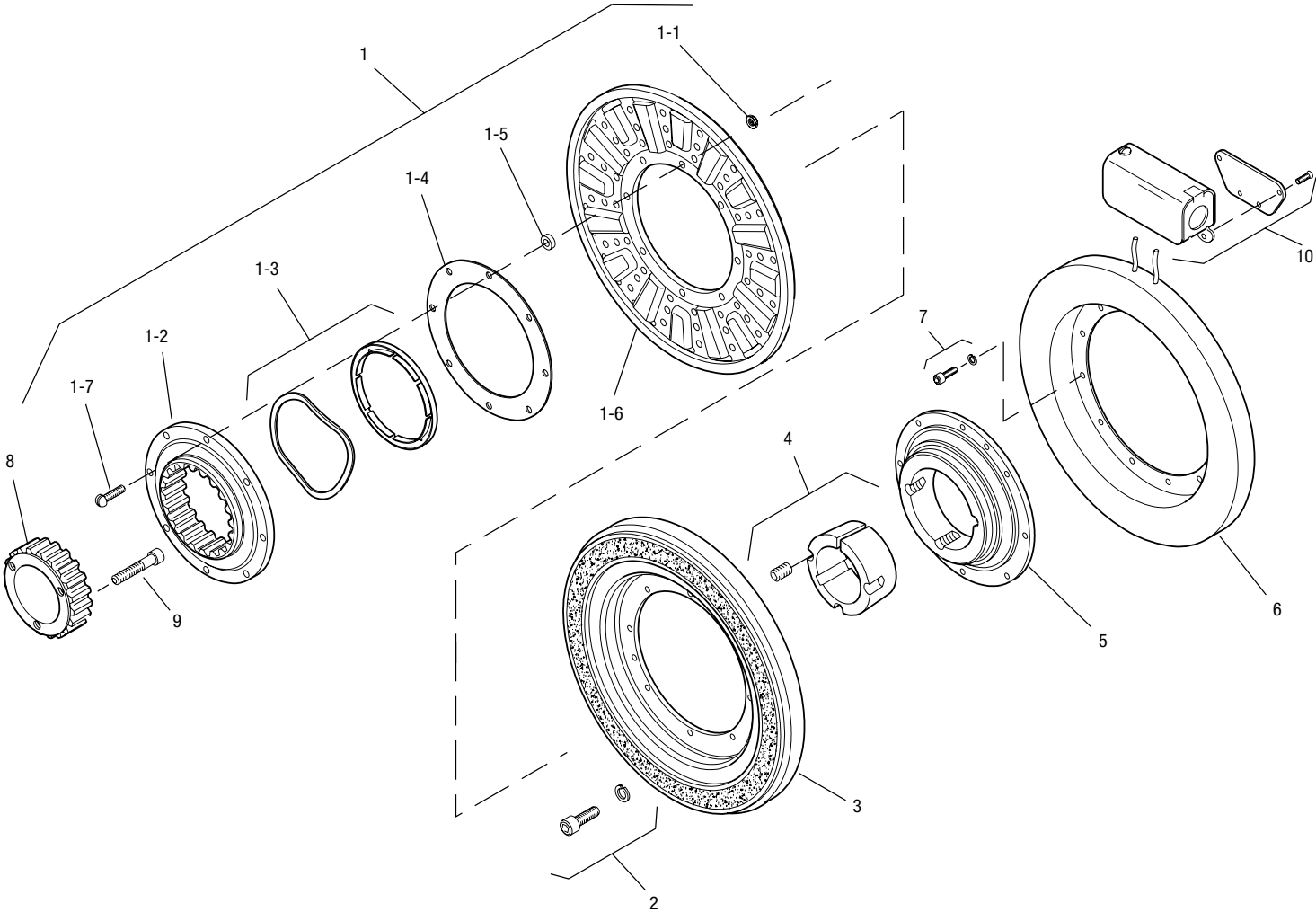
Drawing I-25627
