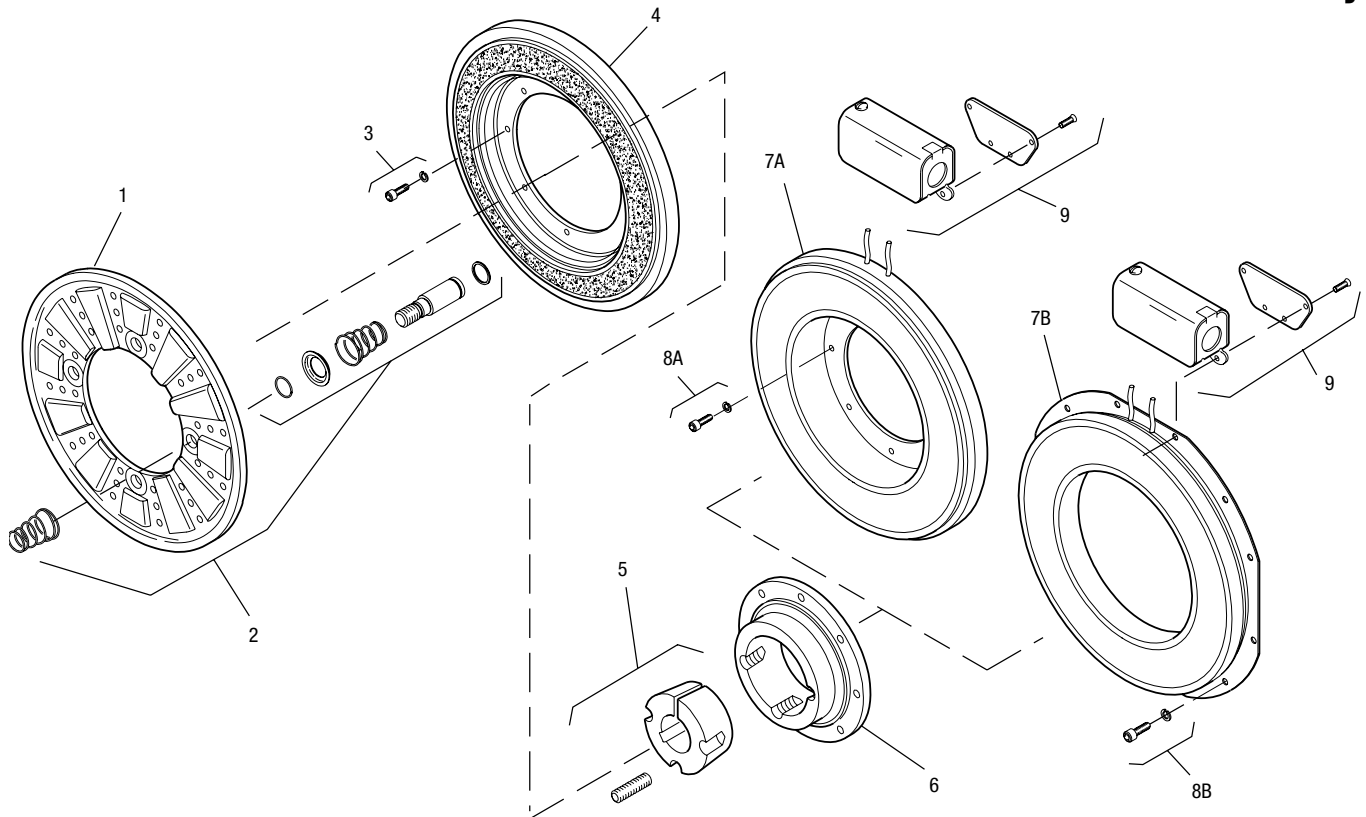
Drawing I-25625
