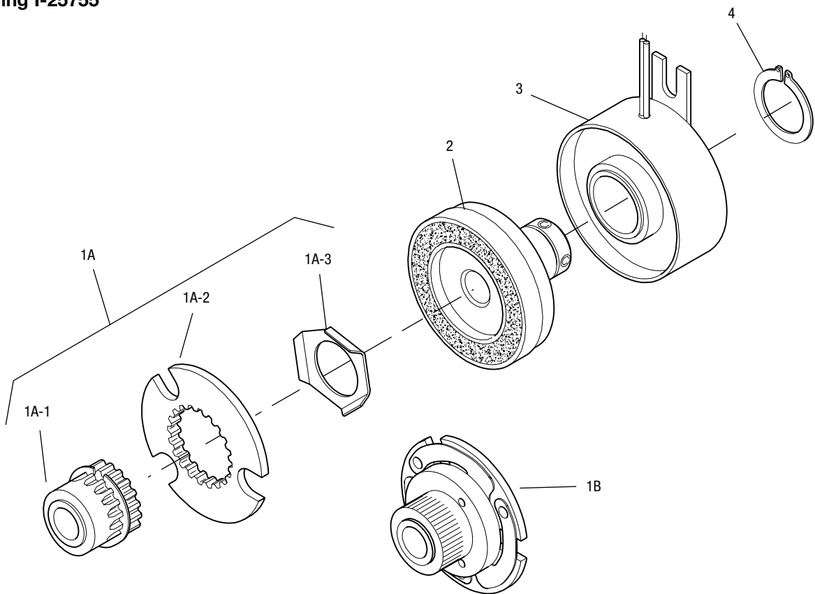
Drawing I-25755
