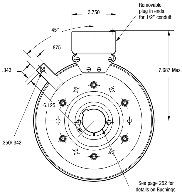
FIELD VIEW
