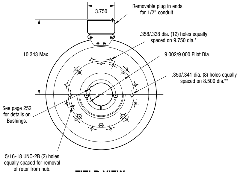
FIELD VIEW
