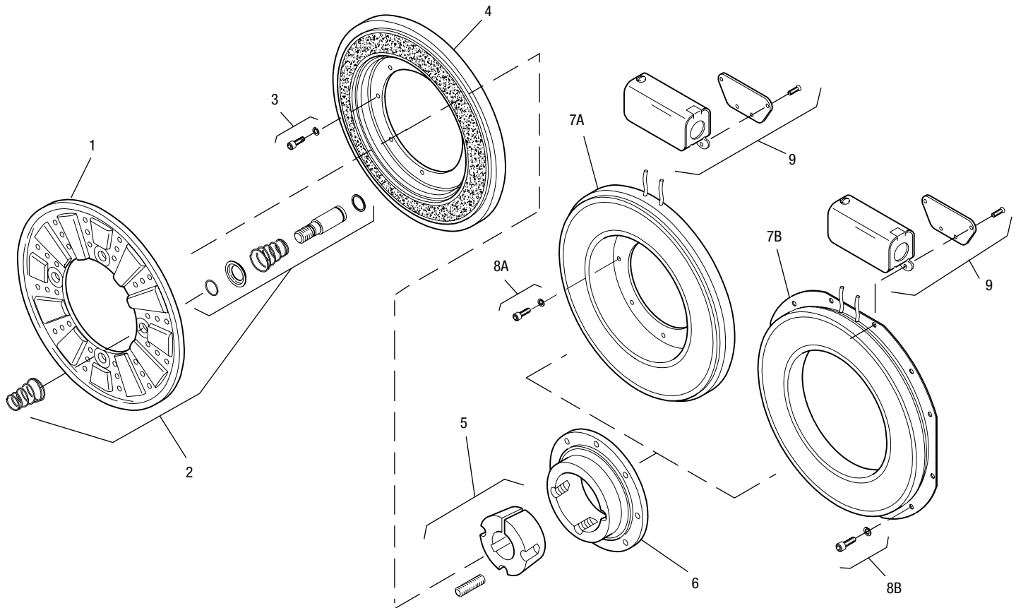
Drawing I-25600
