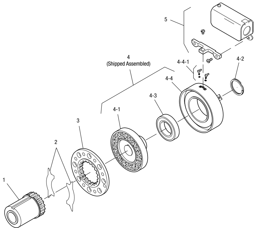
Drawing I-25696
