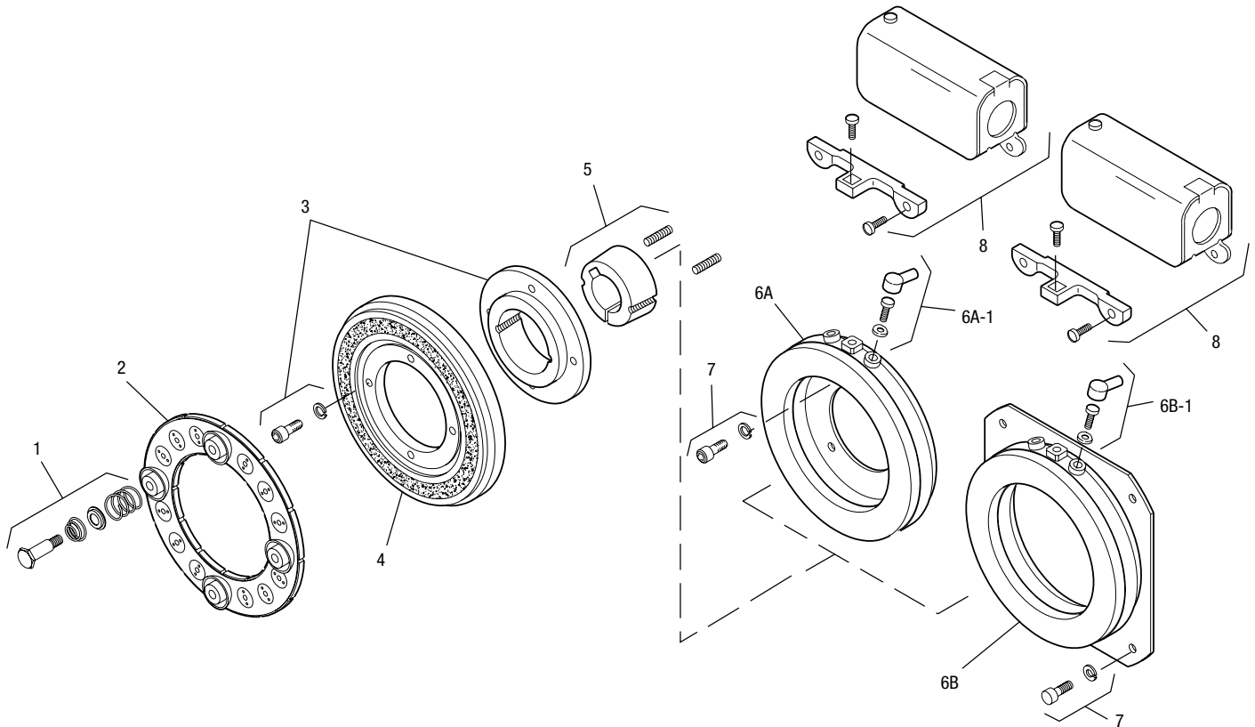
Drawing I-25749
