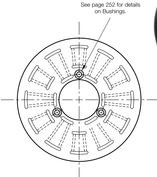
ARMATURE VIEW
