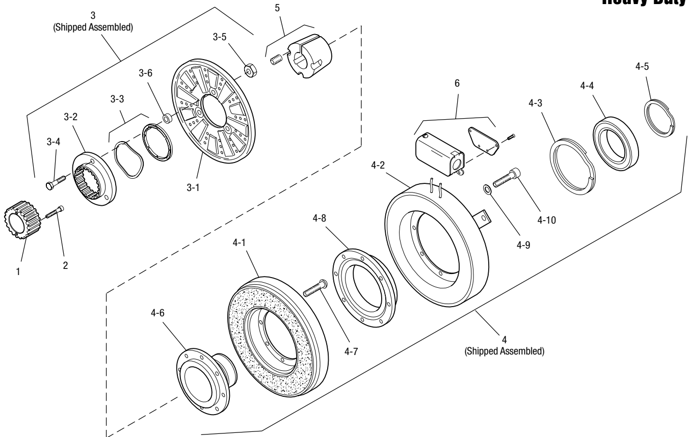
Drawing I-25597
