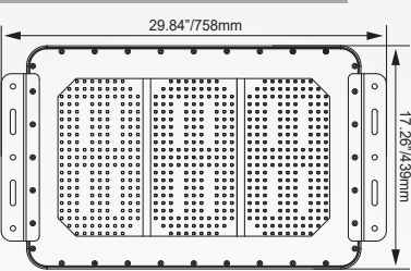
3-DIGIT 2D VIEW
