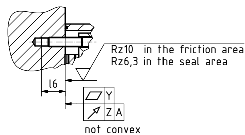
View X without centering
