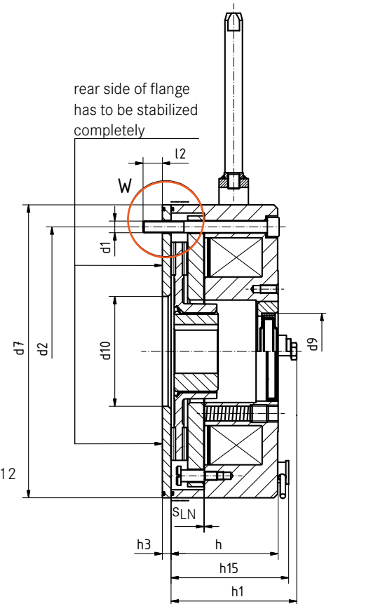
View W with centering
