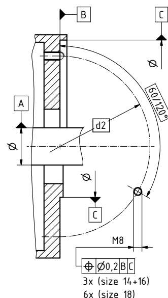
View X without centering
