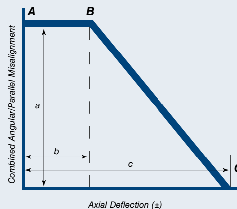
Allowable Misalignments for Disc Couplings
