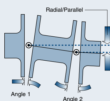
Angular & Radial Misalignment in "Combination"
