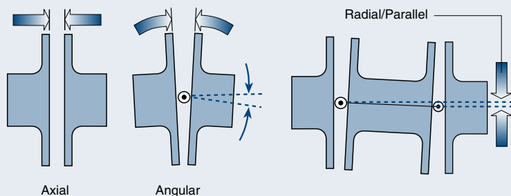
Definition of Misalignments
