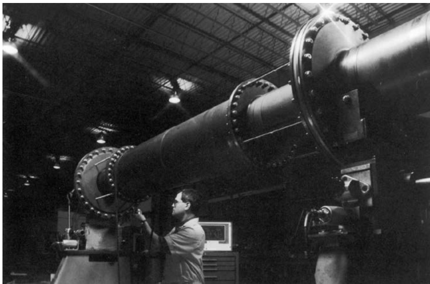
Assembly balancing of a S23-10 Ameriflex coupling for the LM-6000 gas turbine
