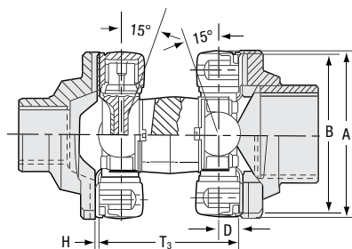
Type “CP” with coupling and without slip – close-coupled (standard maximum working angle: 15°)
