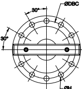
10 Bolt Flange Design with Face Key
