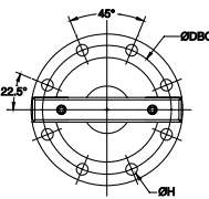
8 Bolt Flange Design with Face Key
