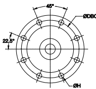
8 Bolt Flange Design
