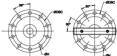
10 Bolt Flange Design
